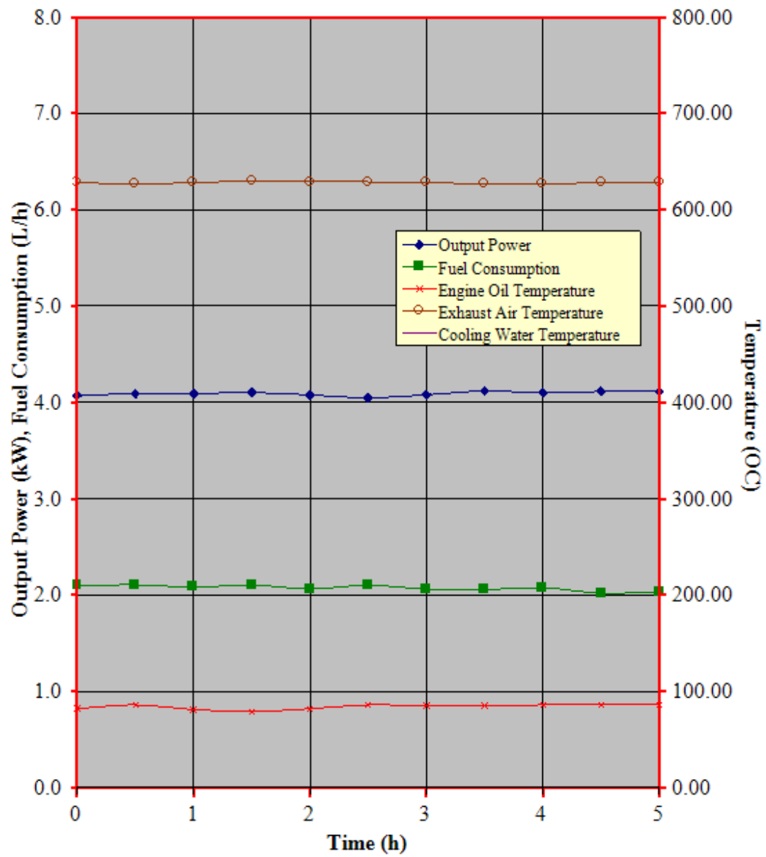
Figure 4. Performance characteristic curves during the continuous running test of the SUMO SE 75M gasoline engine
