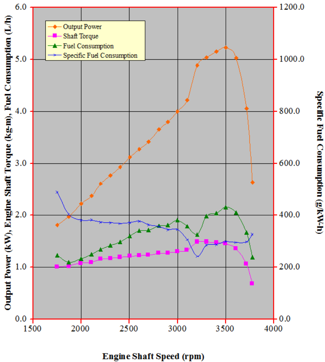
Figure 3. Performance characteristic curves of the SUMO SE 75M diesel engine
